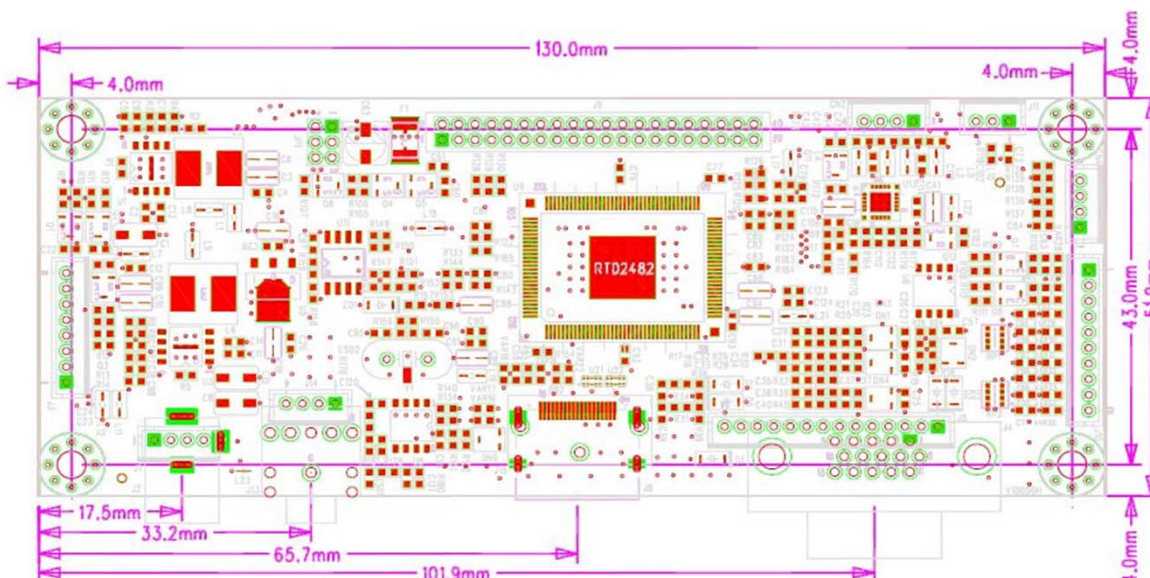
AD board
