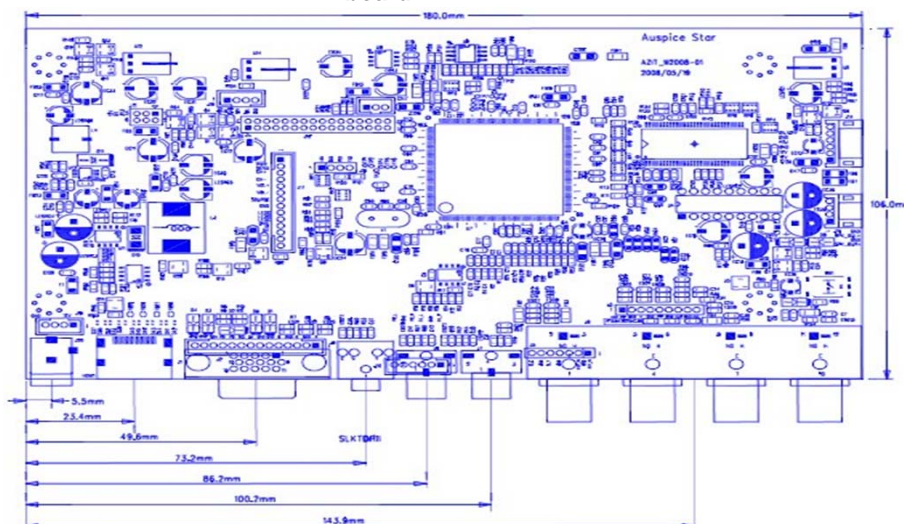
AD board
