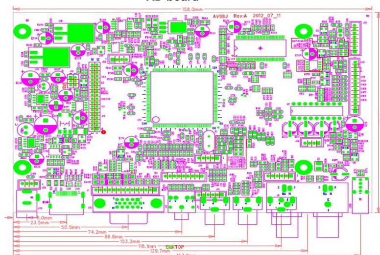
AD board
